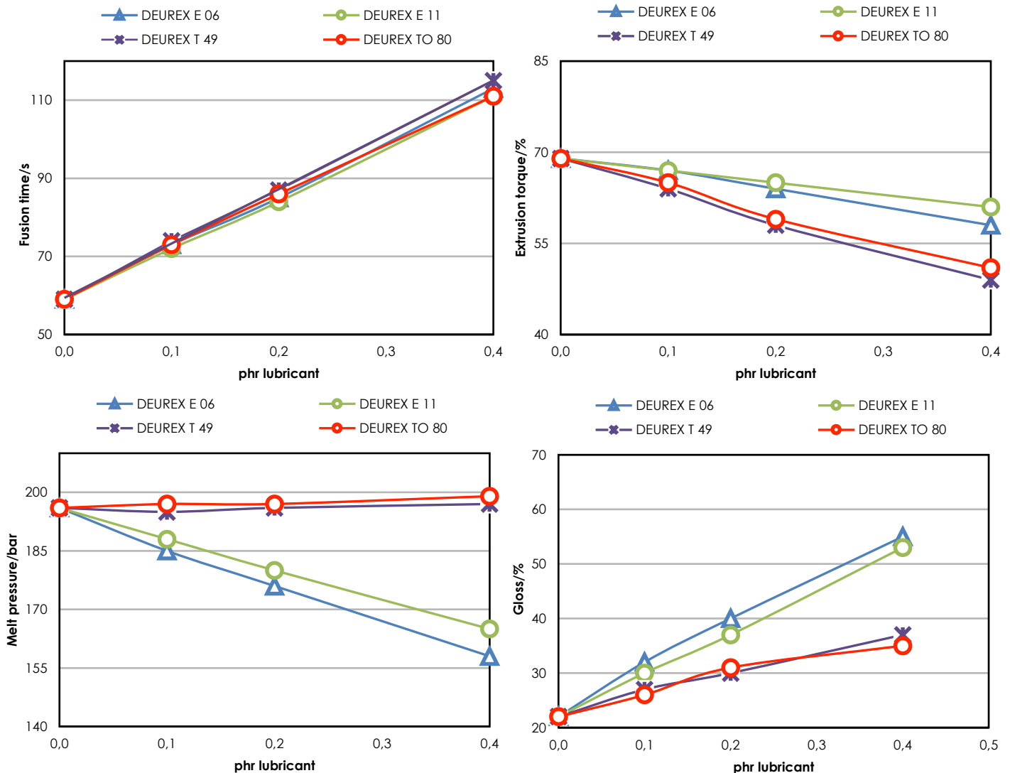
Fig. 1 to Fig. 4 Influence of the dosage of DEUREX® E 06 in comparison to E 11, T 49 and TO 80 on fusion time (Fig. 1), extrusion torque (Fig. 2), melt pressure (Fig. 3) and gloss (Fig. 4)
